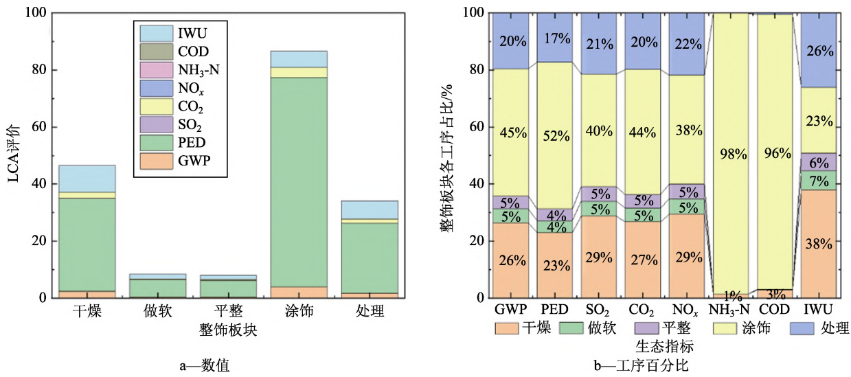
图 6 整饰板块 LCA Fig. 6 LCA results of finishing plate
